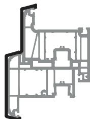
3316 416 gr/m Al cover cap mullion
