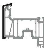
3312 260 gr/m Al cover cap sash
