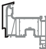
3312 260 gr/m Al cover cap sash
