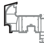
3314 317 gr/m Al cover cap sash
