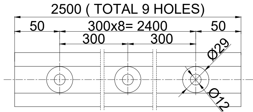
Screw Holes Details (2500mm)
