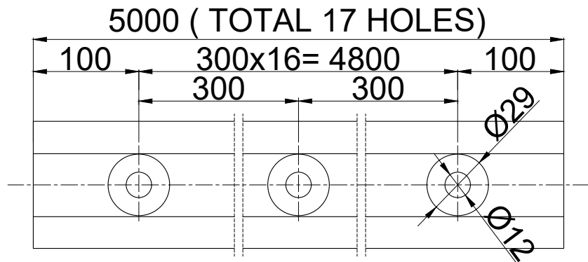
Screw Holes Details (5000mm)
